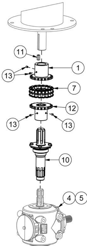
1 3/8" Keyway or Spline Shaft
