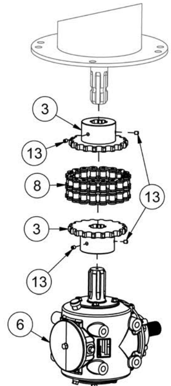
1 3/4" Spline Shaft
